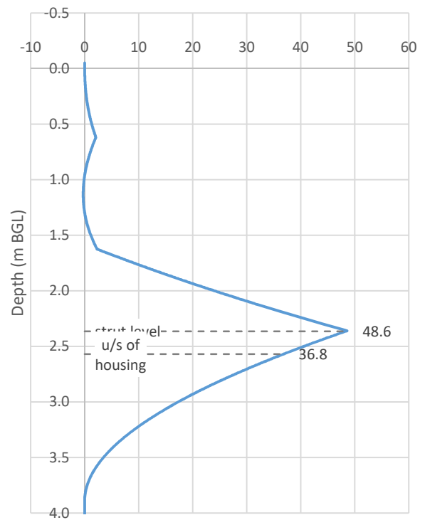
Kicking Moment (kNm per end)
